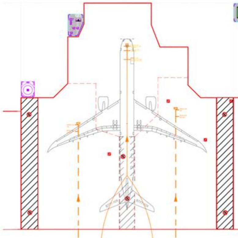
Sample illustration of MARS layout with a parked Code E aircraft
