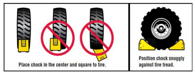
Sample of proper wheel chock placement
